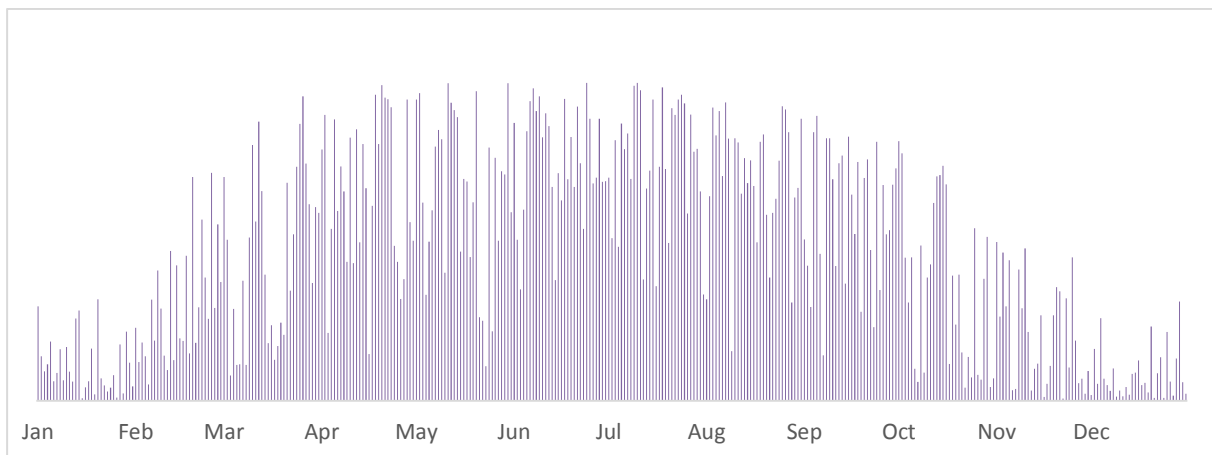
Figure 13: PV energy production simulation for 2014 on Orkney [7]
